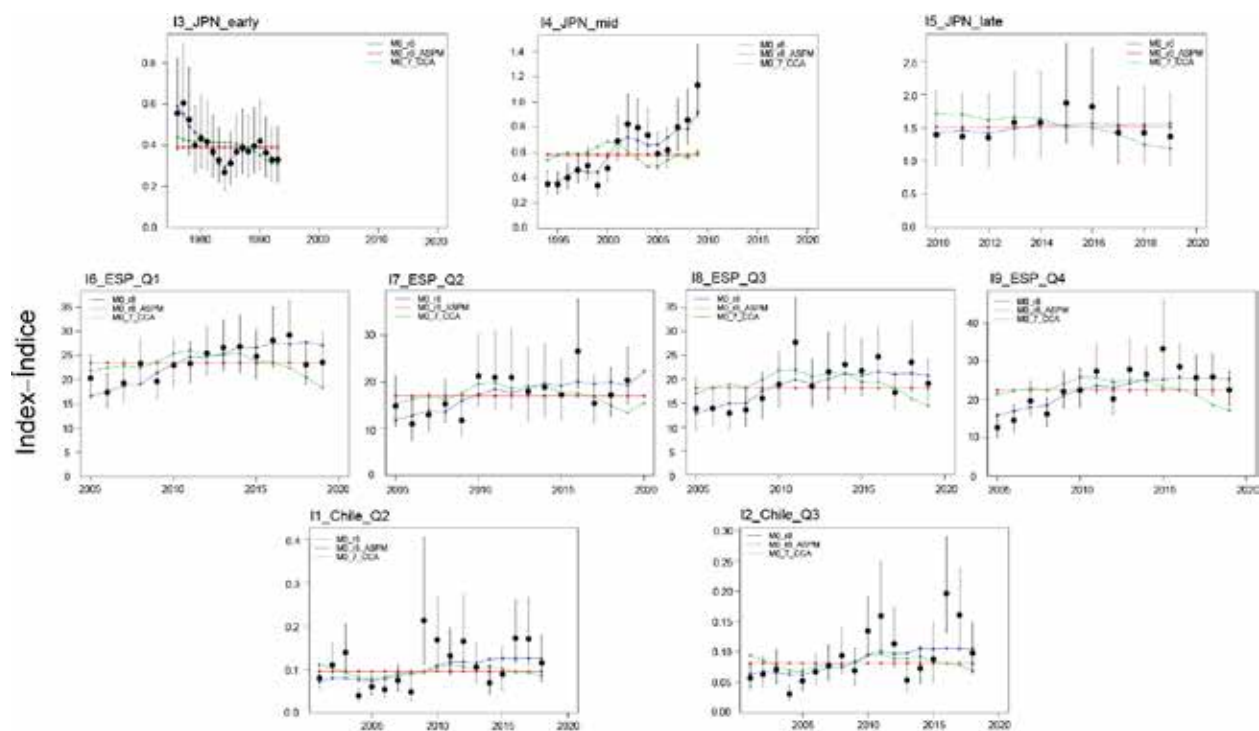
FIGURE 11c. Fit to the indices of abundance of the initial reference model M0 and its ASPM and CCA diagnostics.
