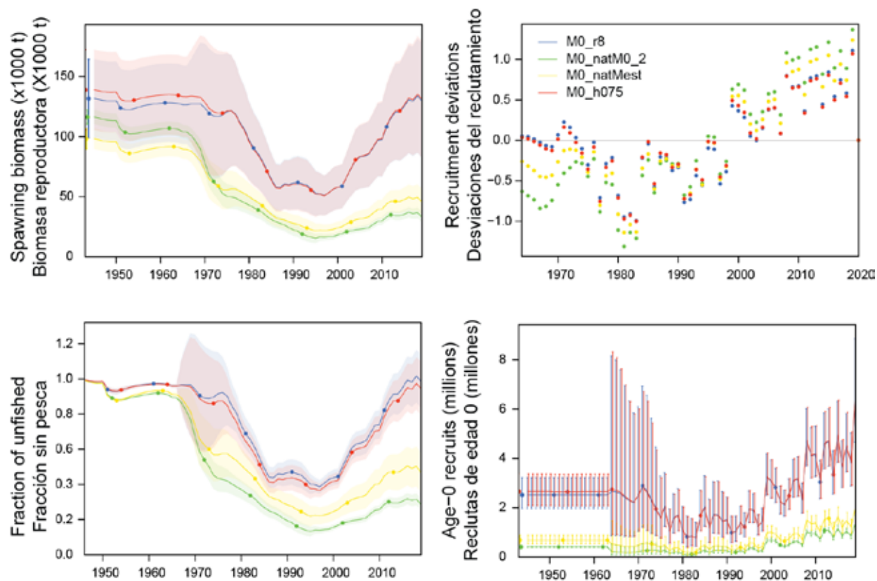
FIGURE 13. Estimated spawning biomass, recruitment deviations, depletion and recruitment estimate for the reference model M0, estimate natural mortality model (M0_natMest), M=0.2 (M0_natM0_2) and h=0.75 (M0_h075) sensitivity models.
