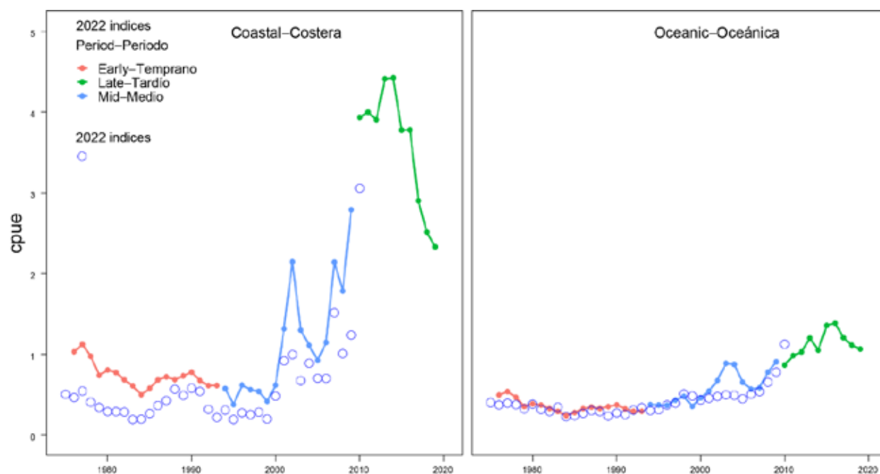
FIGURE 7. Comparison of the Japanese indices from the 2011 assessment and from SAC-13 INF-M, aggregated into the coastal and offshore area.
