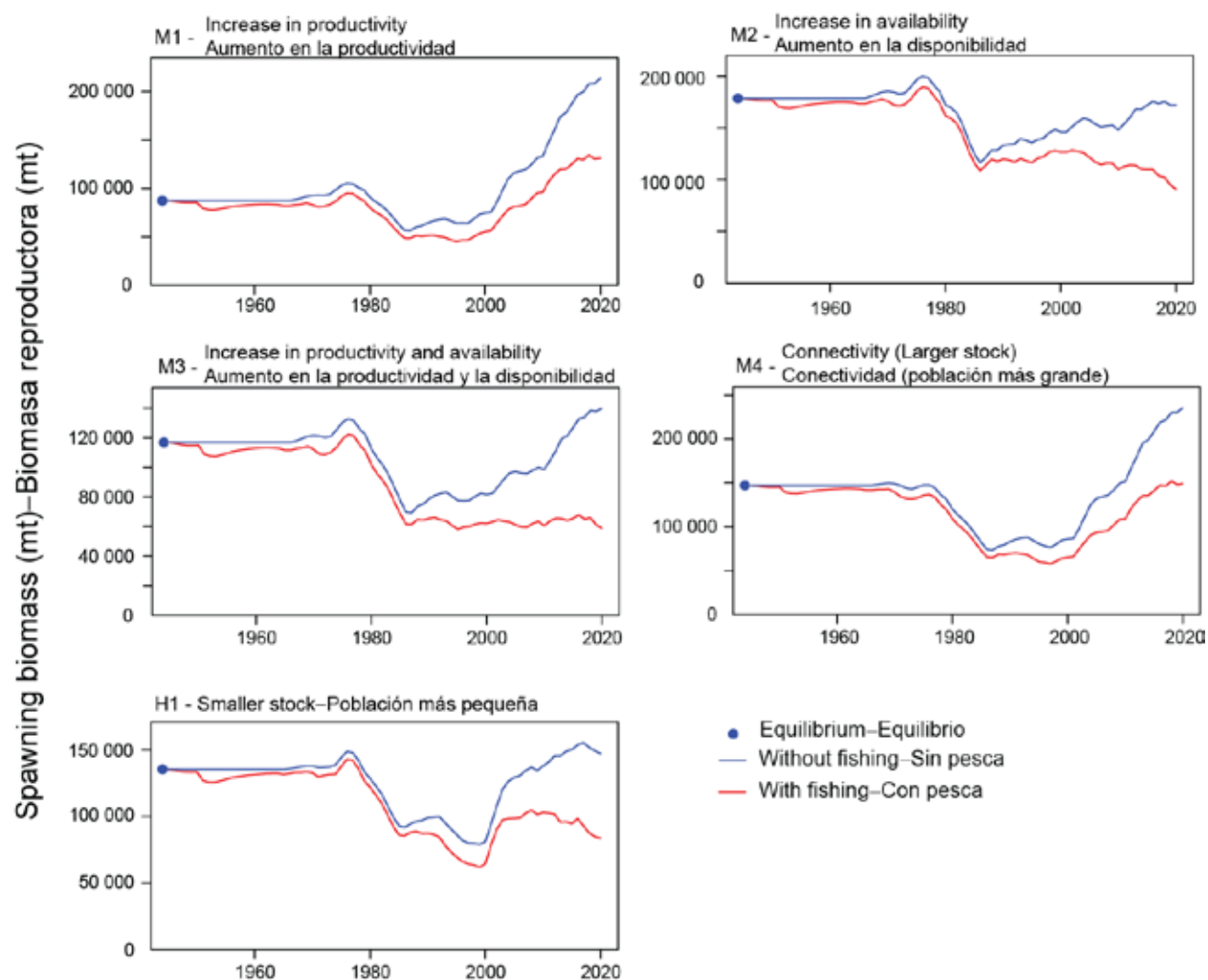
FIGURE 20. Fisheries impact: estimated trends in spawning biomass, with (red line) and without fishing (blue line), from fits of models corresponding to the four hypotheses that explain the simultaneous increase in indices of abundance and catches and the model corresponding to the stock structure hypothesis H1 (north boundary at 5°S). Note that M4 corresponds to the stock structure hypothesis H3 (western boundary at 170°W). The area between the red and the blue line represents the impact of the fisheries on the spawning biomass.
