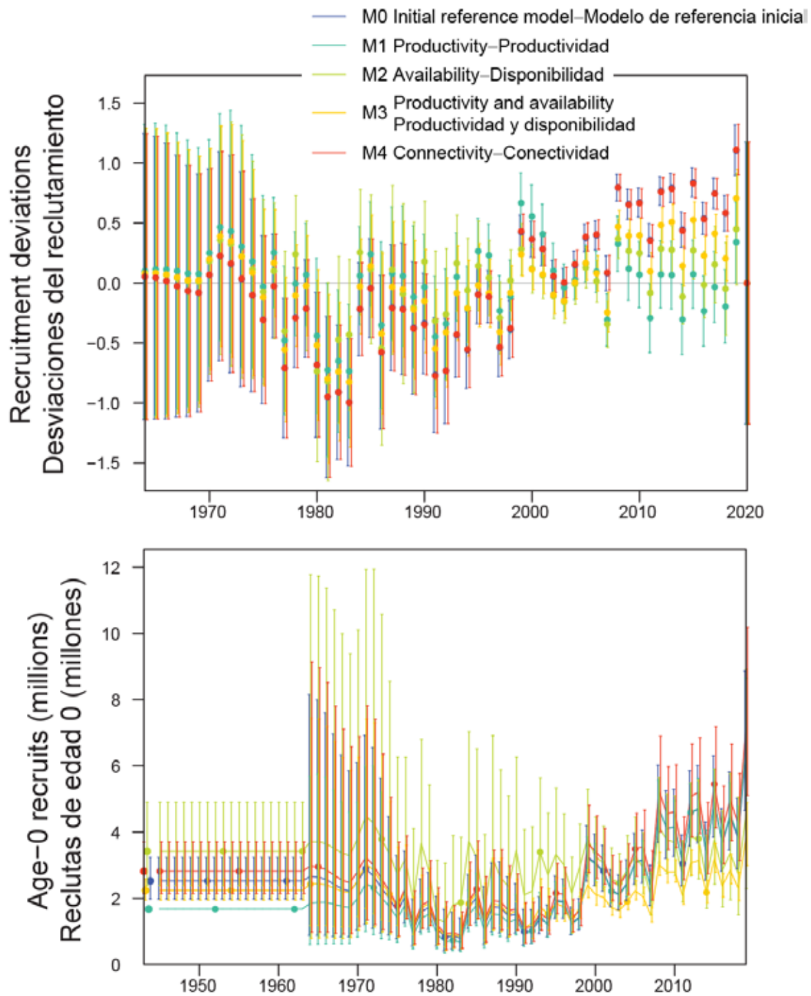
FIGURE 14. Top: recruitment deviations, Bottom: absolute recruitment estimates for the initial reference model M0, and the models corresponding to the four hypotheses that explain the simultaneous increase in indices of abundance and catches.
