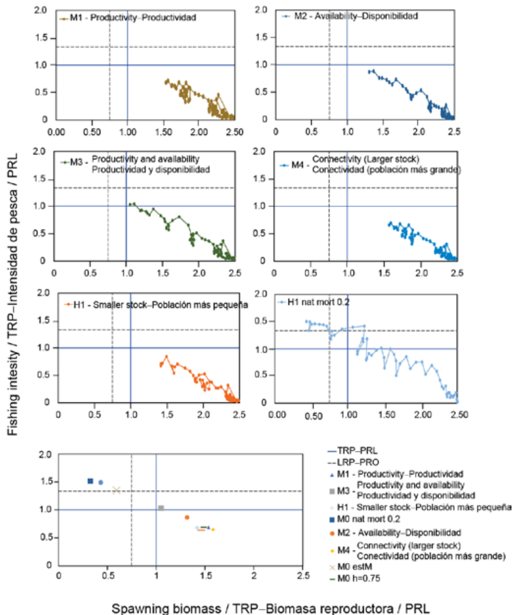
FIGURE 19. Phase plots: Estimated spawning biomass relative to the biomass target reference point ( 40\%SSB_{F=0} ) versus fishing intensity relative to the suggested target reference point ( F40\% ) for the models corresponding to the four hypotheses that explain the simultaneous increase in indices of abundance and catches and the model corresponding to the stock structure hypothesis H1 (north boundary at 5^{\circ}S ). Note that M4 corresponds to the stock structure hypothesis H3 (western boundary at 170^{\circ}W ). The dashed lines correspond to the LRP of F20\% and 20\%SSB_{F=0} .
