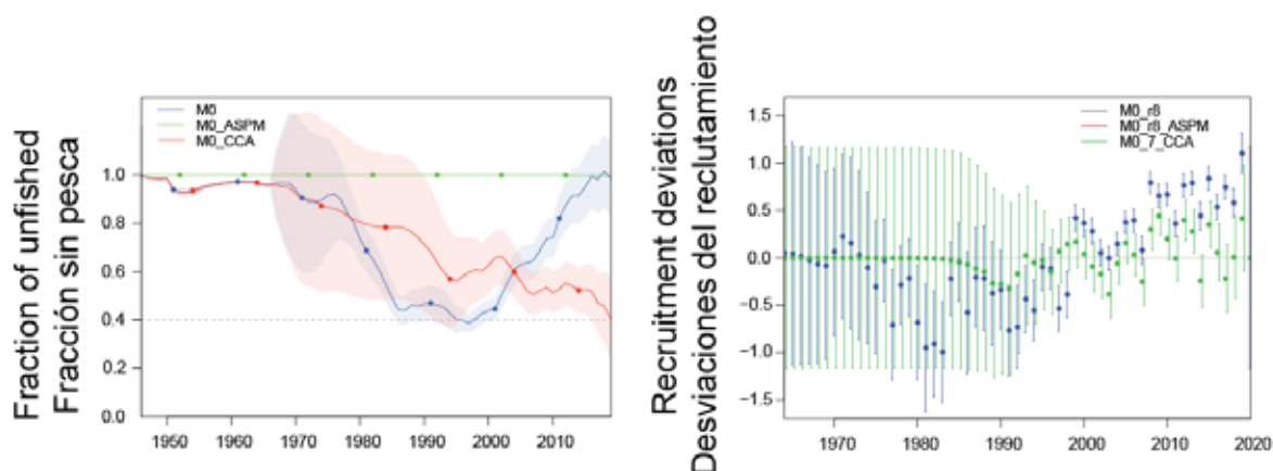
FIGURE 11b. Spawning biomass ratio ( SSB_t/SSB_{F=0,t} ) and recruitment deviations for the initial reference model M0 and its age structure production model (ASPm) and catch curve analysis (CCA) diagnostics.
