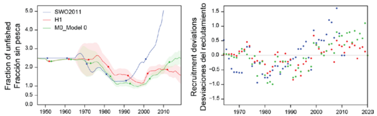
FIGURE 12. Estimated spawning biomass, recruitment deviations, for the 2011 assessment, update model (H1) and initial reference model M0 .
