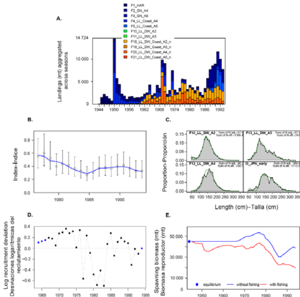
FIGURE A2.1 Model 1B: Catches 1945- 1993 (A); fit to the I3_JPN_early longline index (B); fits to the length composition data (C); estimates of log recruitment deviations (D), Estimated spawning biomass trajectory with and without fishing (trajectory of the spawning biomass of a simulated population of swordfish was never exploited), the area between the red and the blue lines is the impact of fishing (E).
