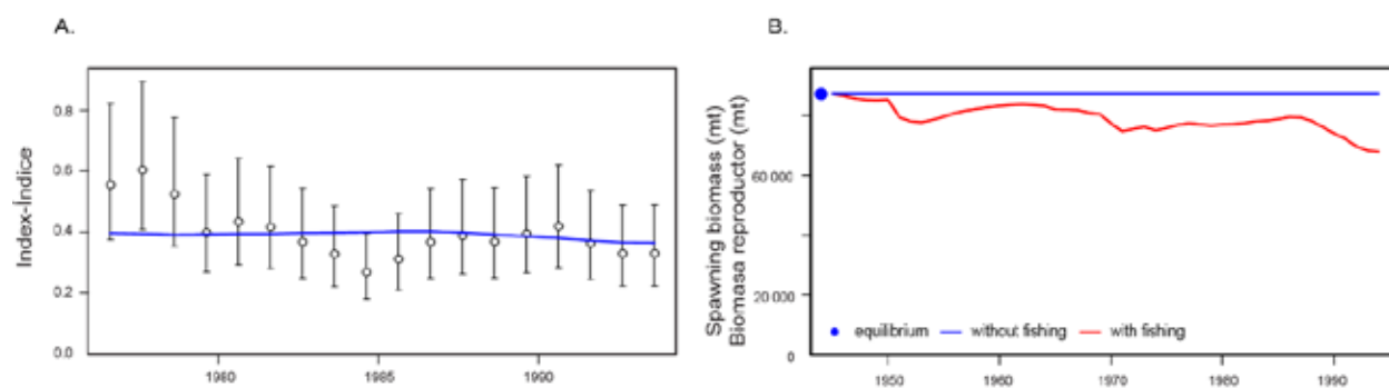
FIGURE A2.2. Model 2: ASPM Early productivity. A: fit to the I3_JPN_early longline index B: Estimated spawning biomass at equilibrium and trajectory with and without fishing.
