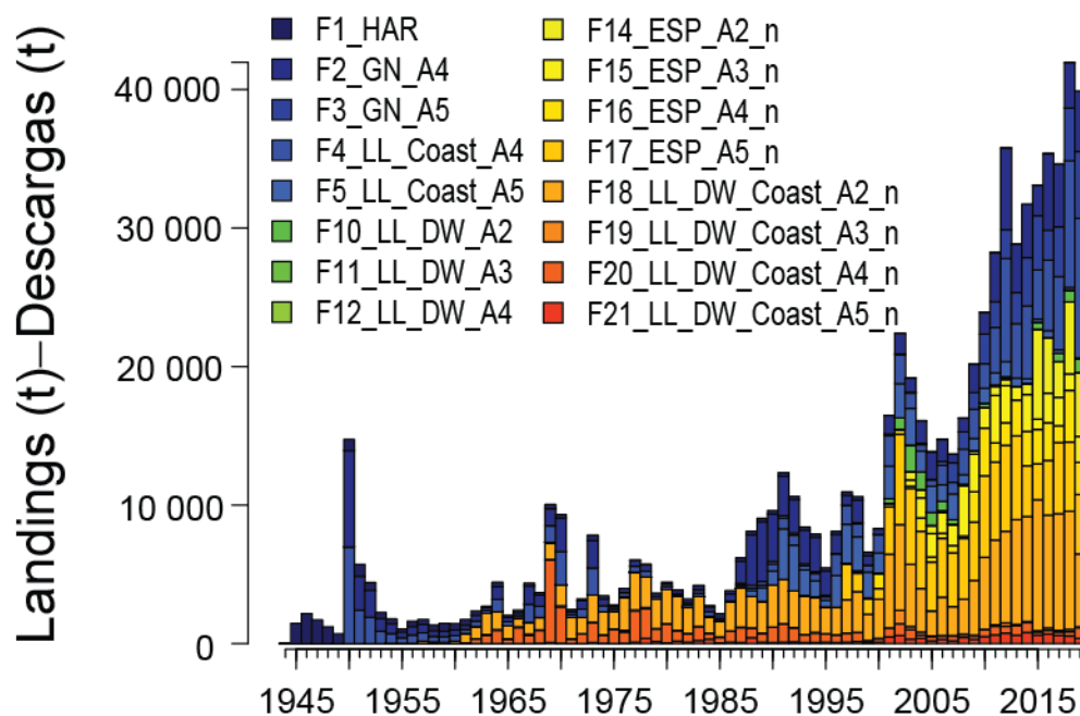
FIGURE 11a. Landings (t), aggregated by fishery and season, for the initial reference model and models that assume the stock structure hypothesis H2.
