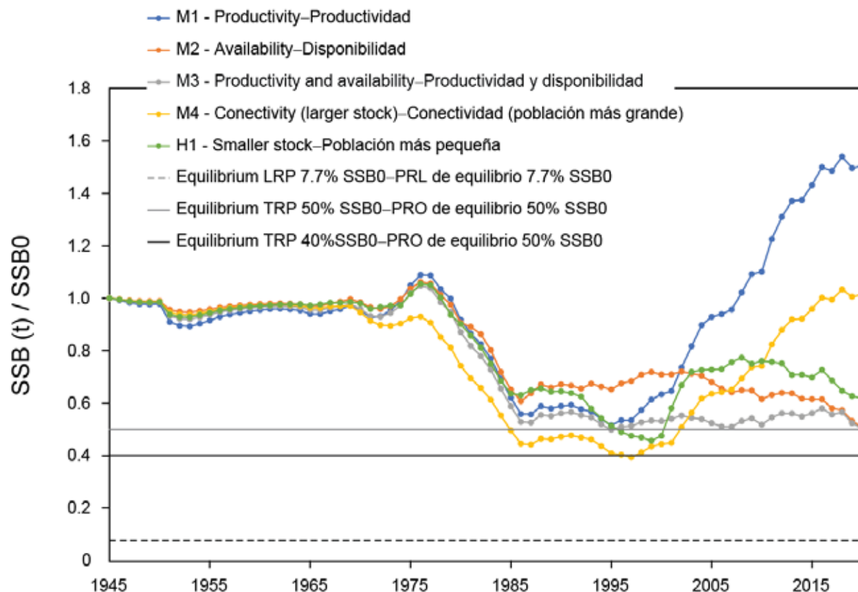
FIGURE 16. Ratio of the estimated spawning stock biomass and the virgin spawning stock biomass (equilibrium) for the models corresponding to the four hypotheses that explain the simultaneous increase in indices of abundance and catches and the model corresponding to the stock structure hypothesis H1 (north boundary at 5°S). Note that M4 corresponds to the stock structure hypothesis H3 (western boundary at 170°W).
