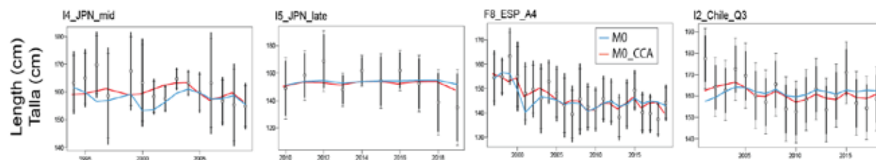
FIGURE 11d. Observed mean length and its expected uncertainty and mean length predicted by the initial reference model and the CCA diagnostic.
