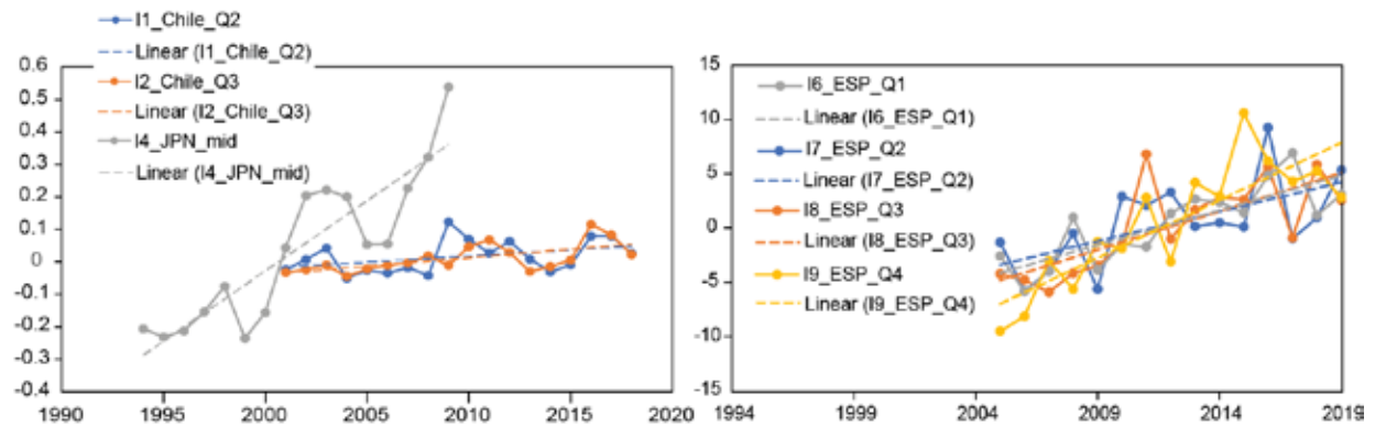
FIGURE A3.1 Time series of estimated catchability deviations (computed as expected index – observed index) for Model 2.
