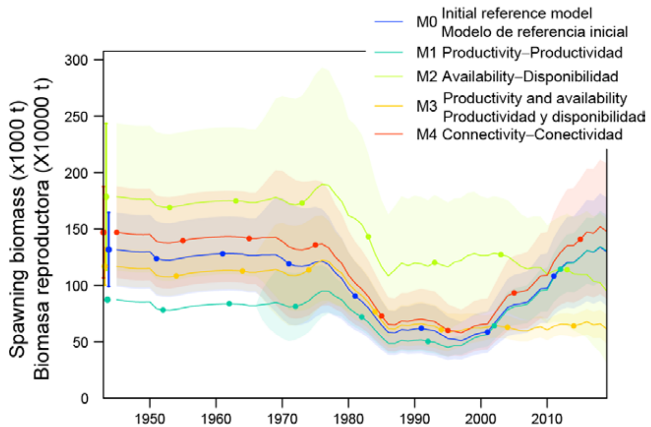
FIGURE 15. Spawning biomass for the initial reference model M0, and the models corresponding to the four hypotheses that explain the simultaneous increase in indices of abundance and catches.
