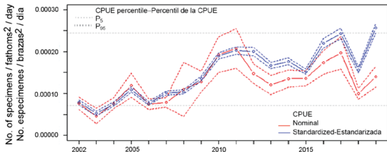
FIGURE 6b. Nominal and standardized gillnet CPUE (and 95% confidence interval for the estimated year effect) for the Chilean fleet (from: Sáez et al. 2020 and Sáez presentation to SWO-01 )
